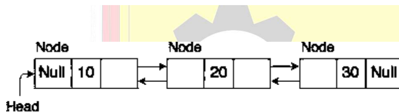
Fig. Doubly Linked List
