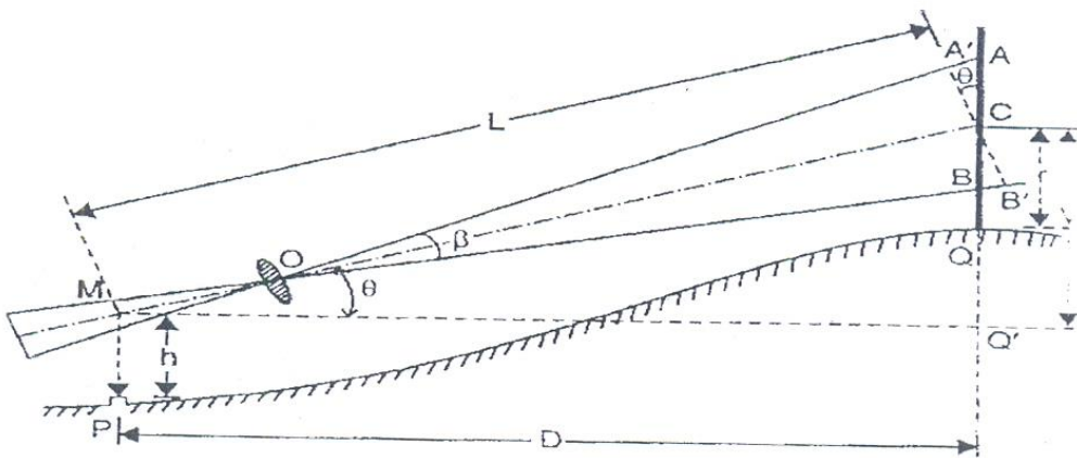
FIG. 22.5. ELEVATED SIGHT : VERTICAL HOLDING.
