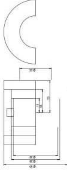
3) Bearing Half
