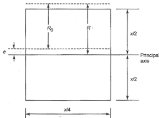
Cross section of tubular frame
